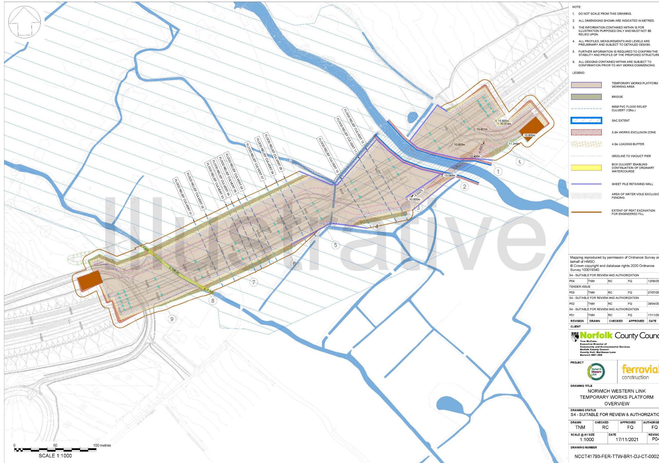
Figure 1.1 Temporary Works Platform Overview
